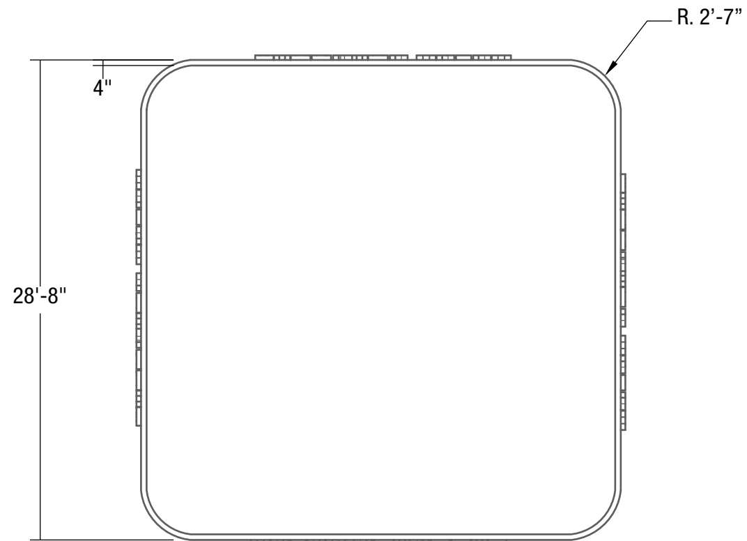
REVERSE PLAN 1/8" = 1'-0"
