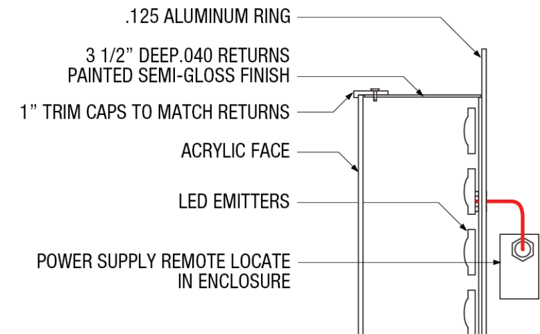
FACE ILLUMINATING SIGNAGE DETAIL NTS
