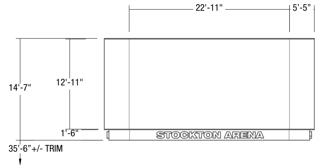
ELEVATION 1/8" = 1'-0"
